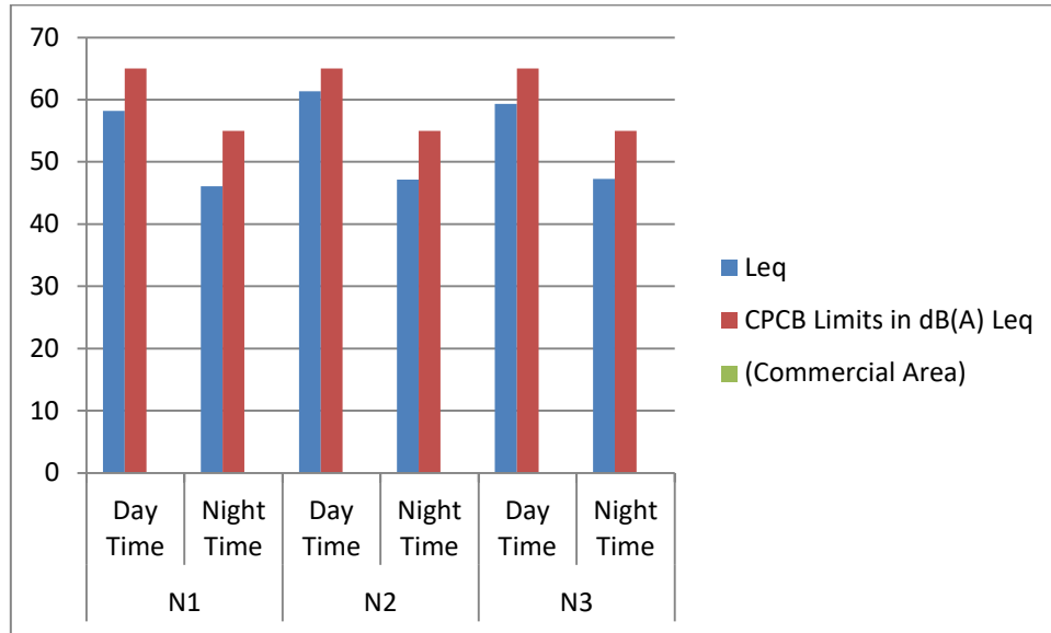
Figure 3.3 Location-wise Variation of CO in Ambient Air Quality
