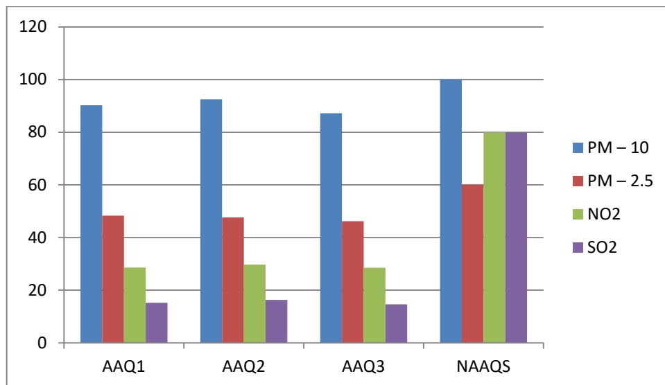
Figure 3.1 Location-wise Variation of Ambient Air Quality (PM 2.5 , PM 10 , SO x , NO x )
